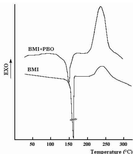
Fig. 1. DSC curves of BMI and BMI+PBO equimolecular mixture
