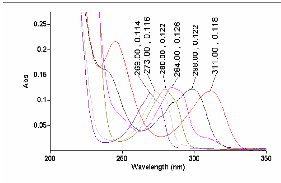
Figure 1. UV spectra for phenol (6.8 mg/L), 2-CP (8.0 mg/L), 4-CP (10.0 mg/L), 2,4-DCP (10.0 mg/L), 2,6-DCP (6.0 mg/L), 2,4,6-DCP (6.0 mg/L), in distilled water at pH = 7.0
